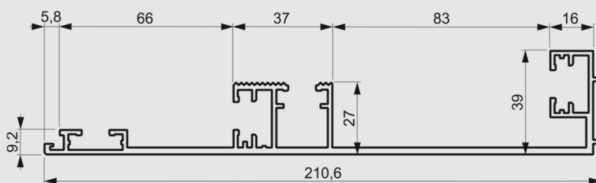
AS 210S Profil de cadre
