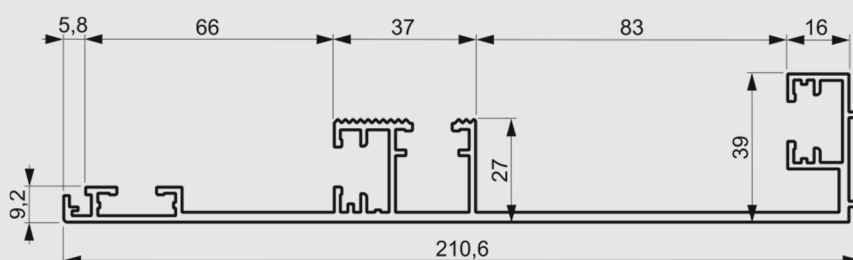
AS 210.1S Profil de cadre
